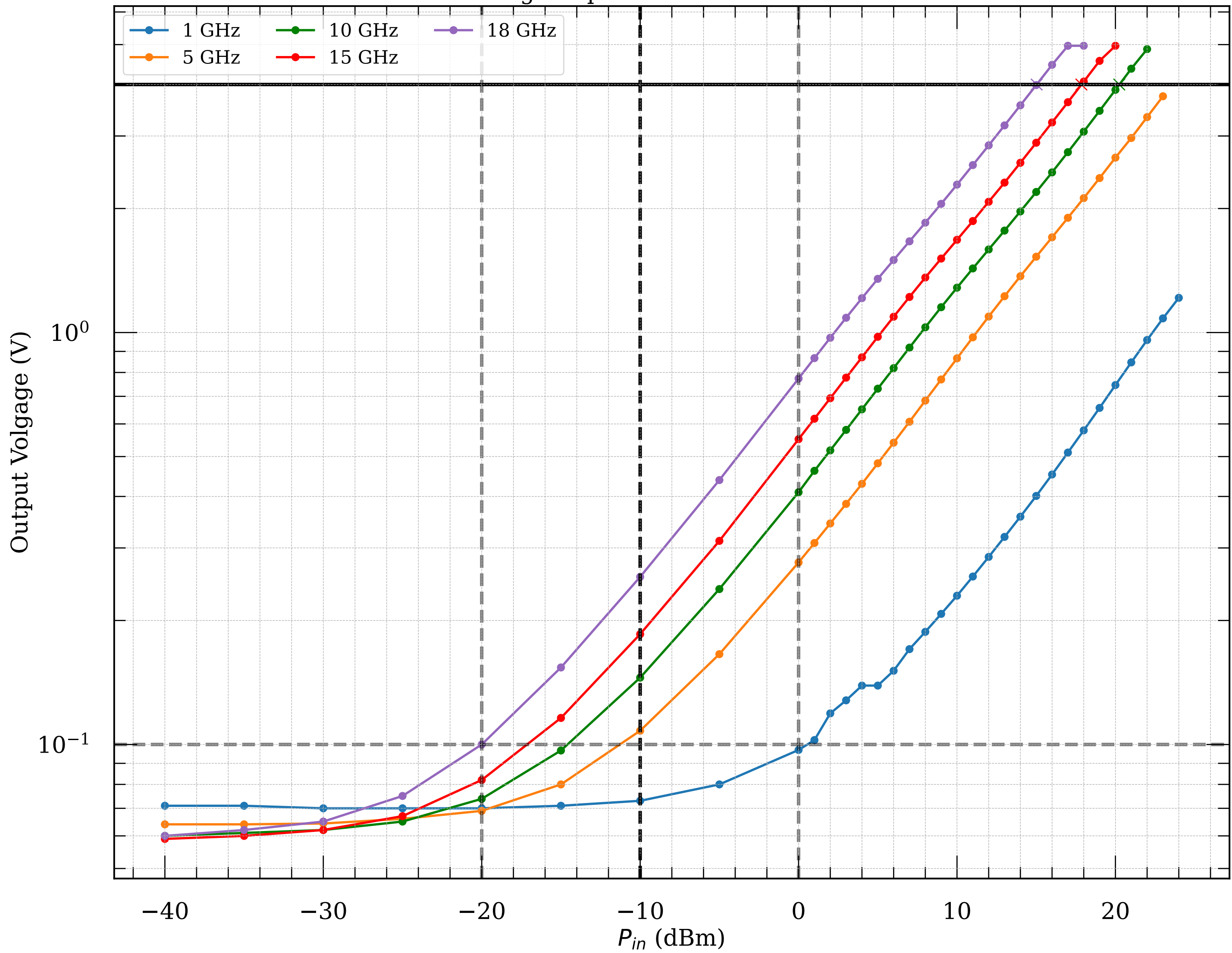
Measured voltage-to-power curve of detector module037
